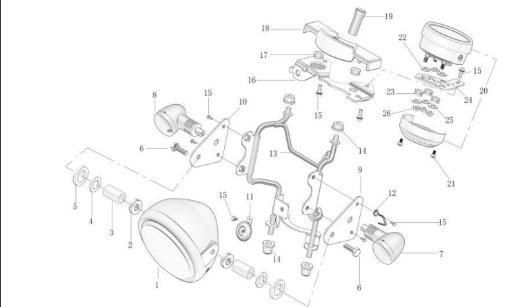
F-14 仪表/前照灯 METER/FRONT HEADLIGHT
