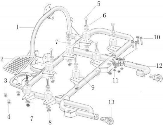
F-20 边车车架/BASKET FRAME
