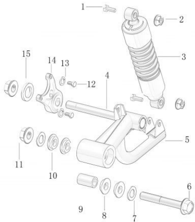
F-19 边车减震/BASKET SHOCK
